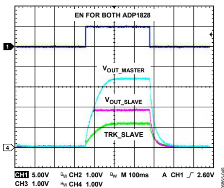
Figure 48. Ratiometric Tracking of Figure 47
