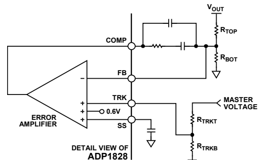
Figure 42. Voltage Tracking
