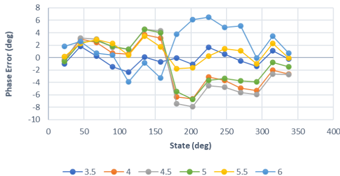
Phase Error (°) vs. State (S12)
