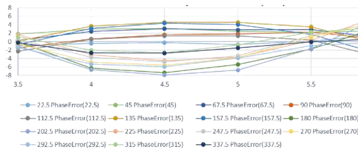
Phase Error compared to ideal (S12)
