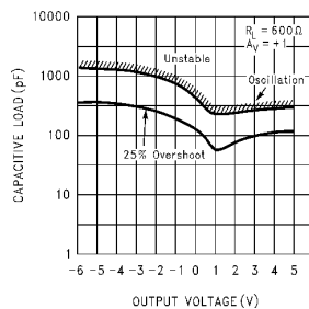
Stability vs Capacitive Load, R_L = 600\Omega
