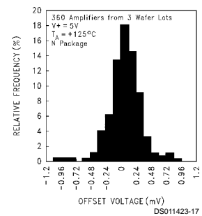
Distribution of LMC6081 Input Offset Voltage ( T_{\text{A}} = +125^\circ\text{C} )
