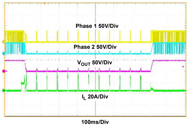
Figure 34. Short-Circuit Waveform
