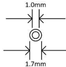
Figure 5: Dimensions of tie-point (left) and mounting hole (right).
