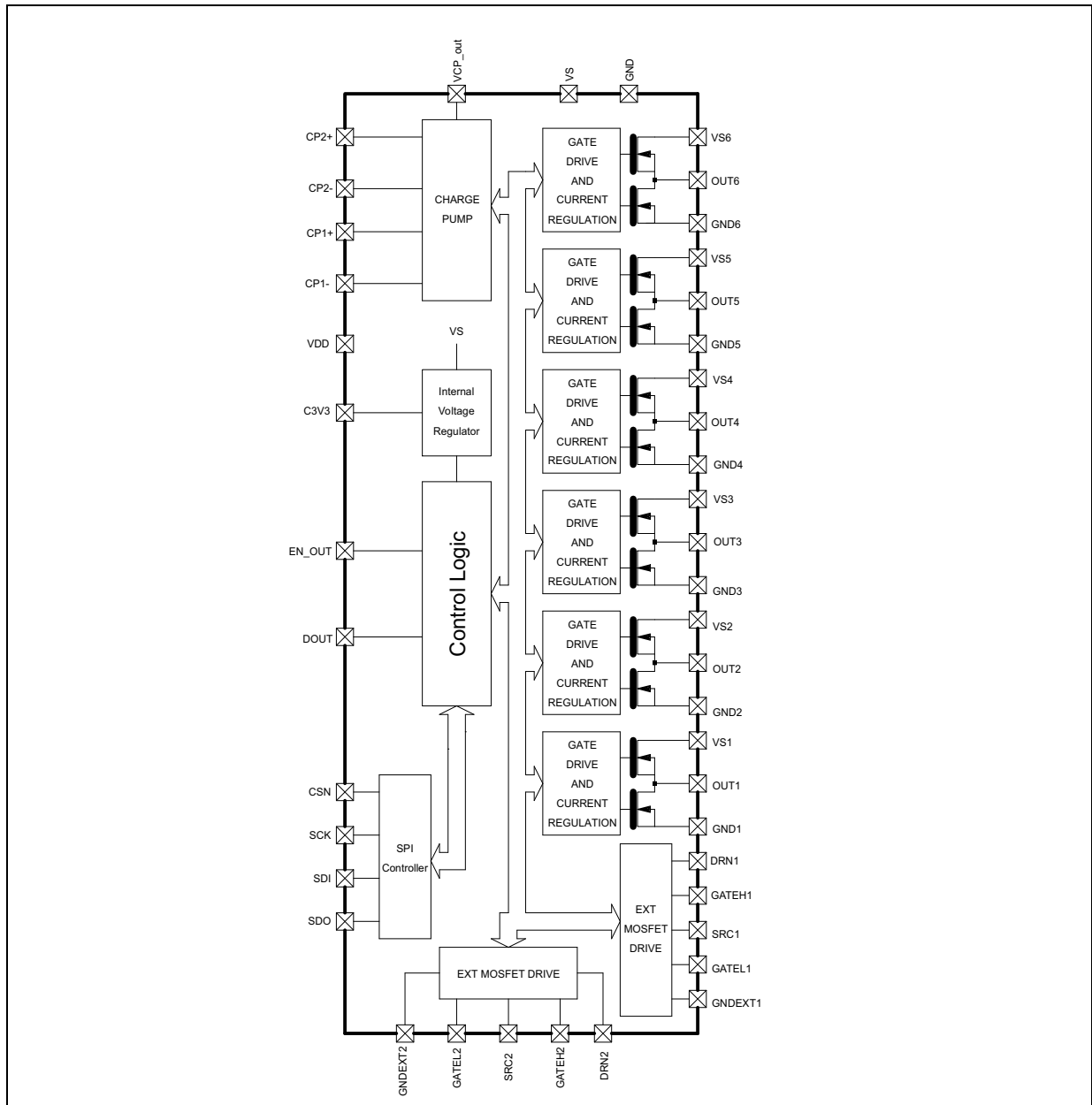
Figure 1. Block diagram
