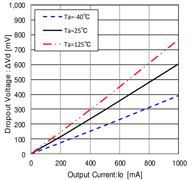
Figure 51. Dropout Voltage ( V_{CC}=V_o \times 0.95V=7.6V )
