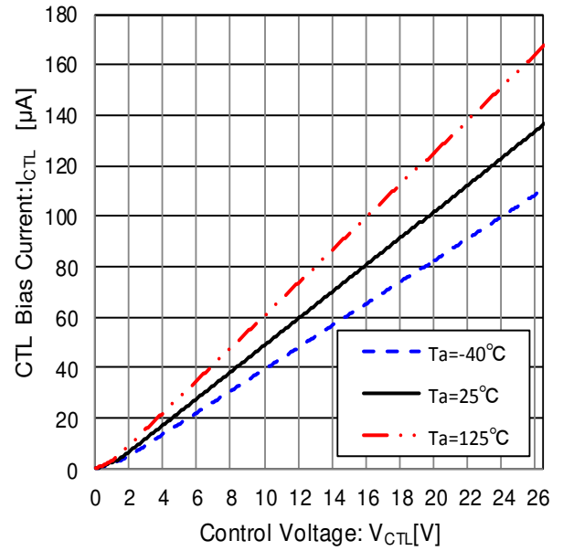
Figure 67. CTL Current vs CTL Voltage
