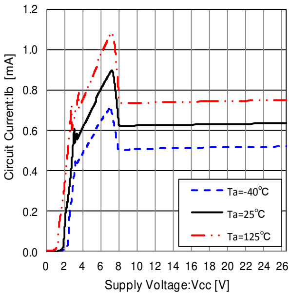
Figure 46. Circuit Current
