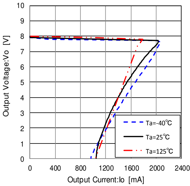
Figure 50. Load Regulation
