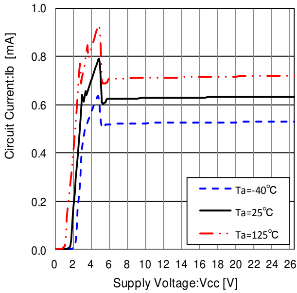
Figure 34. Circuit Current
