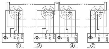
Connection diagram
