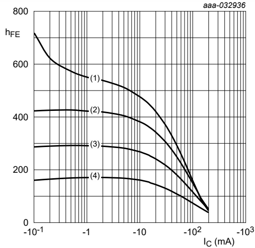
V_{CE} = -5\text{ V} (1) T_{amb} = 175\text{ °C} (2) T_{amb} = 100\text{ °C} (3) T_{amb} = 25\text{ °C} (4) T_{amb} = -40\text{ °C}
