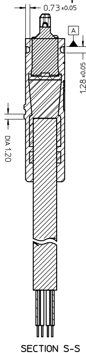
SECTION S-S
