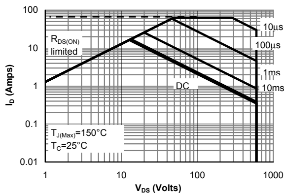
Figure 11: Maximum Forward Biased Safe Operating Area for AOW15S60 (Note F)
