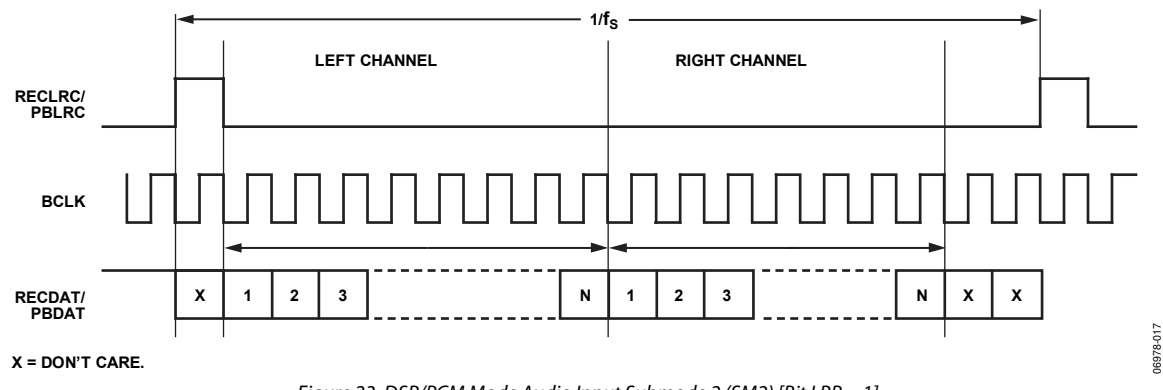
Figure 23. DSP/PCM Mode Audio Input Submode 2 (SM2) [Bit LRP = 1]
