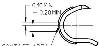
CONTACT AREA ON DIMPLE DETAIL2 SCALE : 20:1
