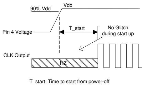
Figure 4. Startup Timing (OE/ST Mode) [9]
