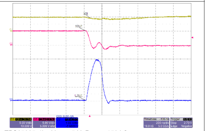
Figure 28. Transient: Thermal Fault Latched
