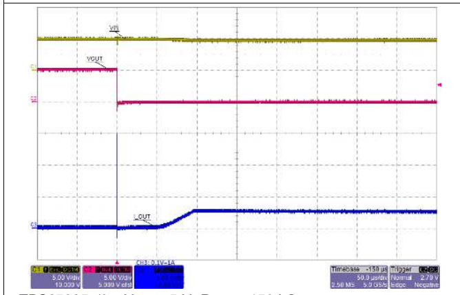
Figure 27. Transient: Thermal Fault Auto-Retry
