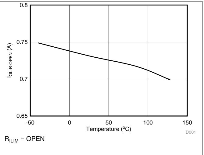
Figure 14. I_{OL-R-Open} vs Temperature
