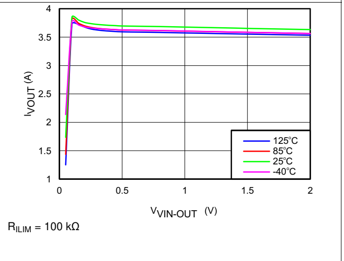
Figure 16. I_{OUT} vs V_{VIN-OUT}
