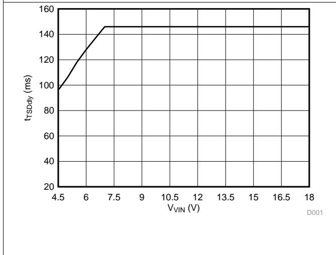
Figure 15. Retry Delay vs V_{VIN}
