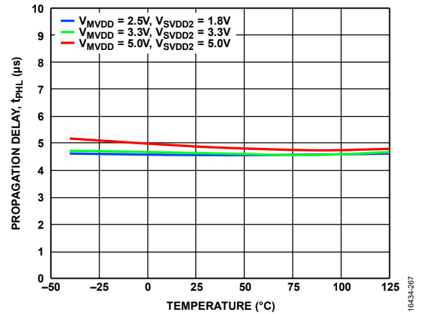
Figure 63. GPIO Channels Propagation Delay ( t_{PLH} ) vs. Temperature at Various Supply Voltages
