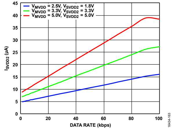
Figure 61. SVDD2 Supply Current ( I_{SVDD2} ) vs. Data Rate on All GPIO Channels at Various Supply Voltages, \overline{MSS} Is High
