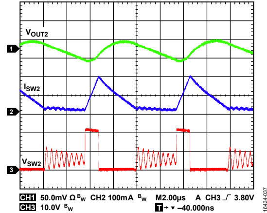
Figure 38. Buck Regulator Discontinuous Conduction Mode Operation Showing I_{L2} , Switch Node Voltage, and Output Ripple, T_A = 25^\circ\text{C} , V_{OUT1} = 21\text{ V} , V_{OUT2} = 5.15\text{ V} , I_{OUT2} = 50\text{ mA}
