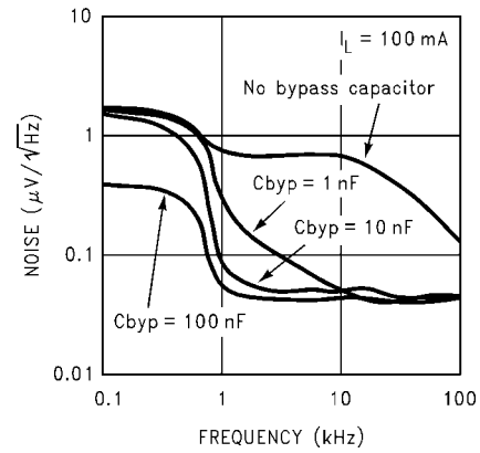
Noise Density
