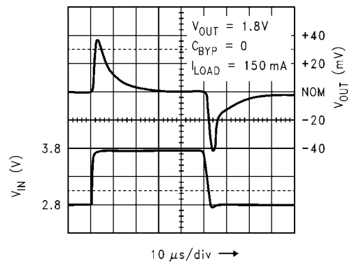
Line Transient
