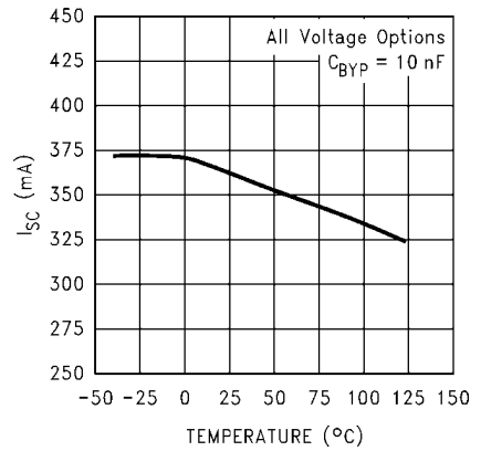
Instantaneous Short Circuit Current
