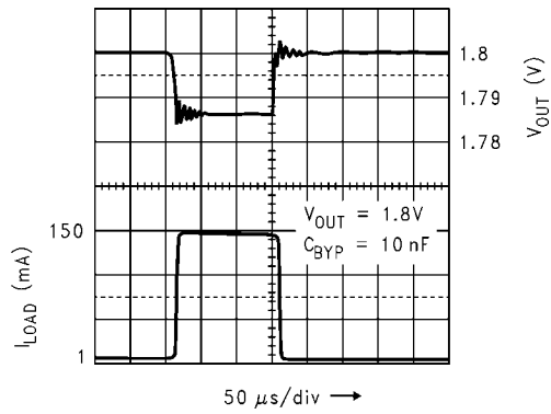
Load Transient
