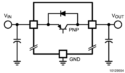
FIGURE 3. Reverse Current Path
