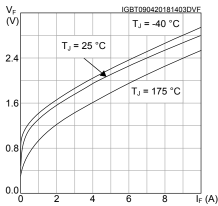
Figure 9. Diode V_F vs forward current
