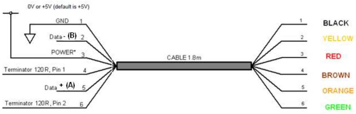
Figure 5.1 USB-RS485-WE Connections
