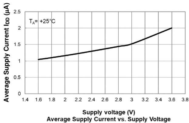
Average Supply Current vs. Supply Voltage
