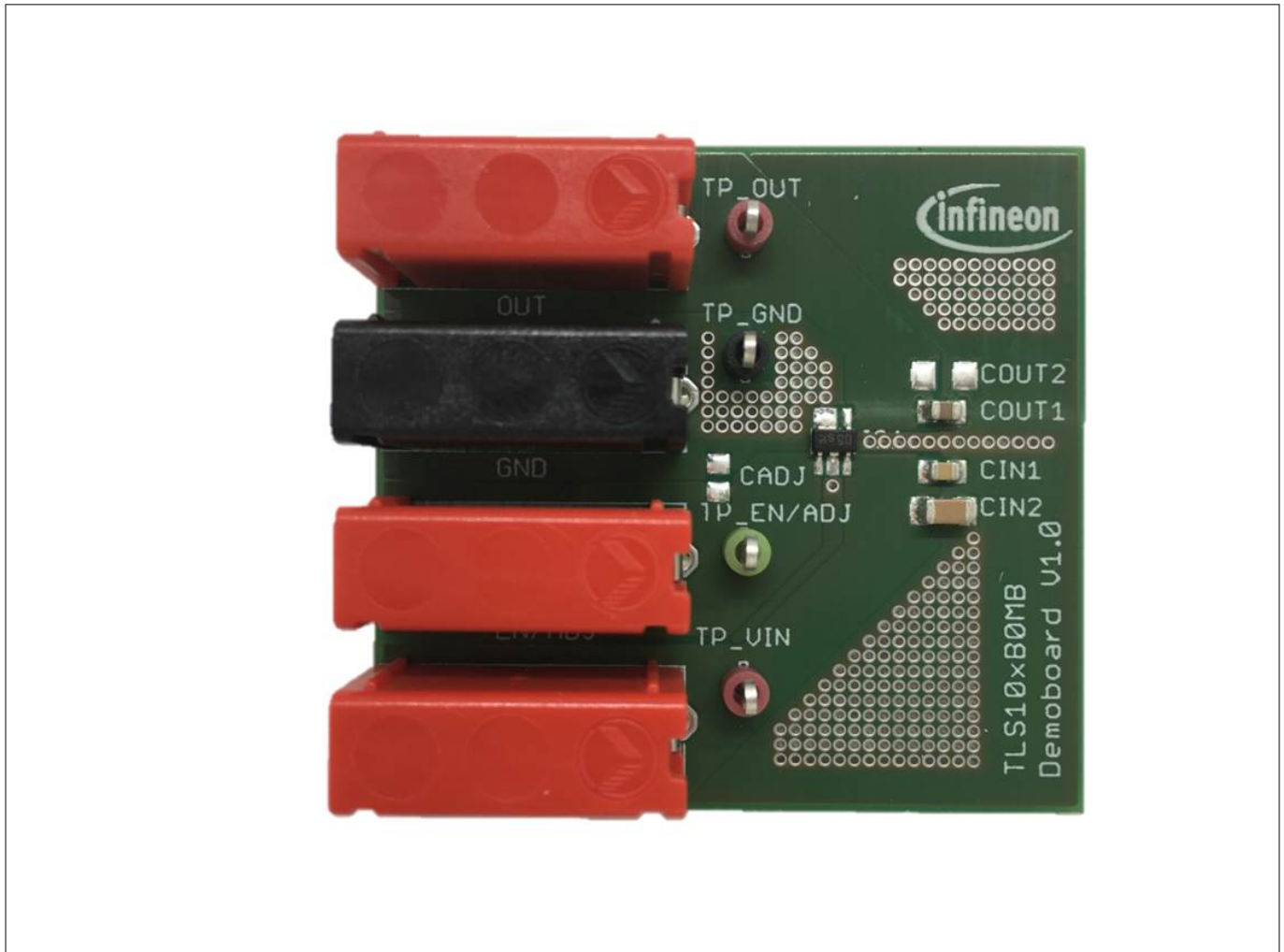
Figure 2 Demoboard
