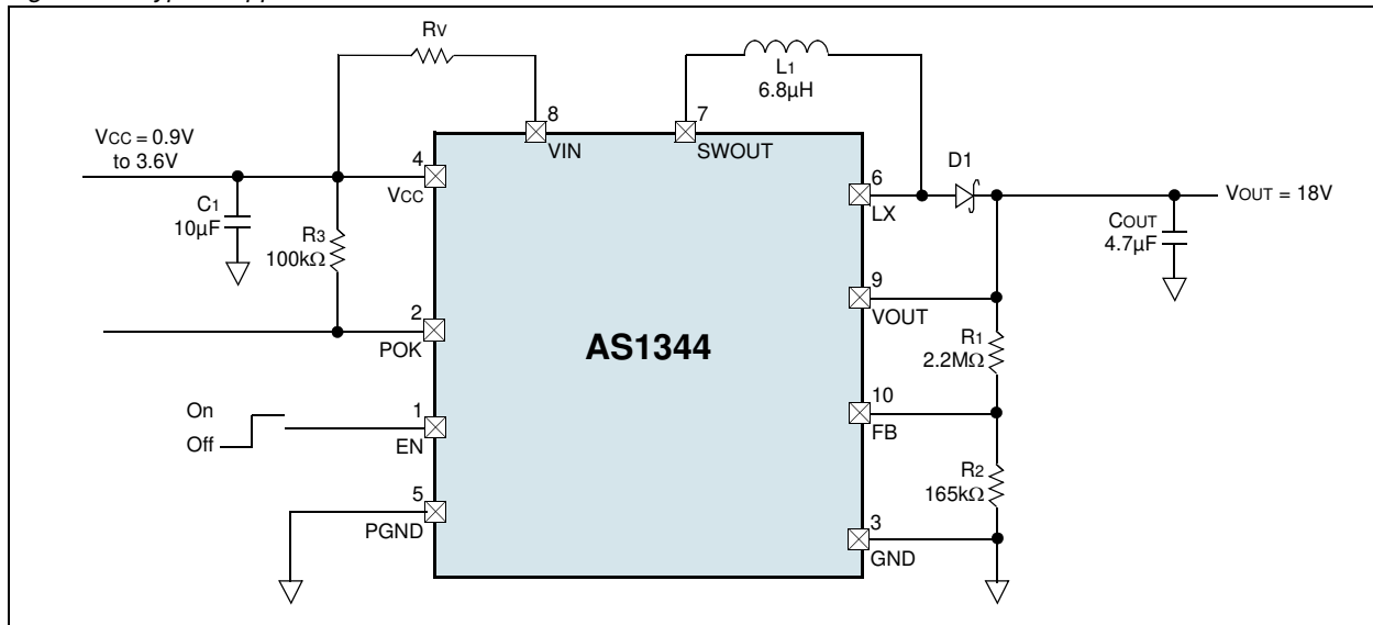
Figure 35. Typical Application
