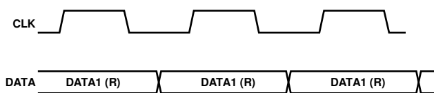
Figure 10. Mono PDM Format
