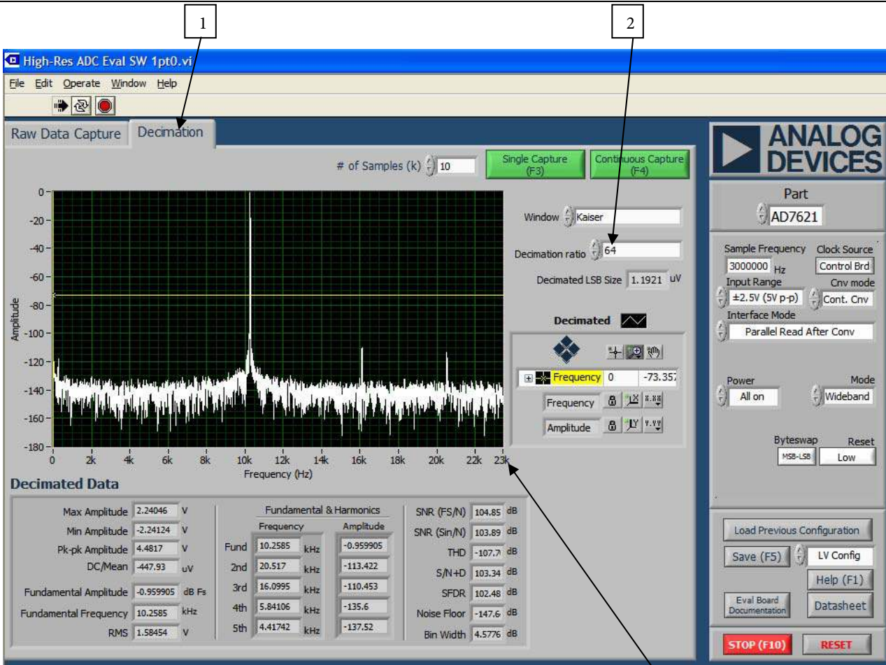
Figure 17 .Decimated FFT
