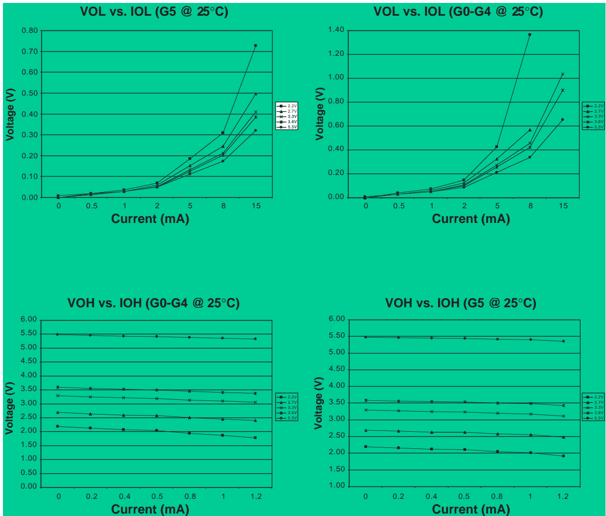
Figure 10: VOL/VOH
