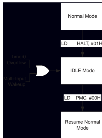
Figure 29: Recommended IDLE Flow
