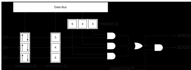
Figure 18: Multi-input Wakeup (MIW) Block Diagram
