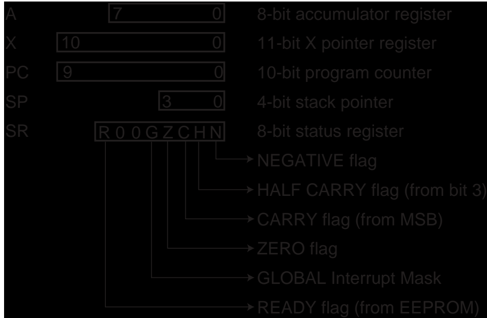
Figure 11: Programming Model
