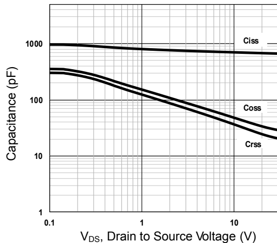
Figure 7. Capacitance Characteristics
