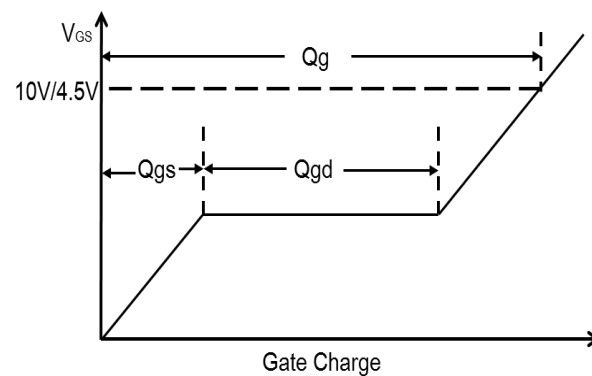
Figure 12. Gate Charge Waveform
