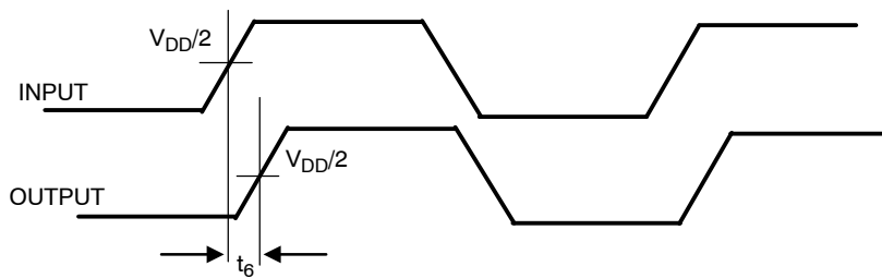
Figure 3. Switching Waveforms
