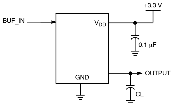
Figure 4. Test Circuit
