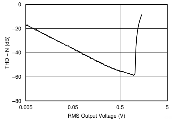
Figure 9-3. THD + N vs RMS Output Voltage
