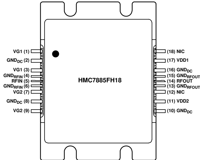
Figure 2. Pin Configuration
