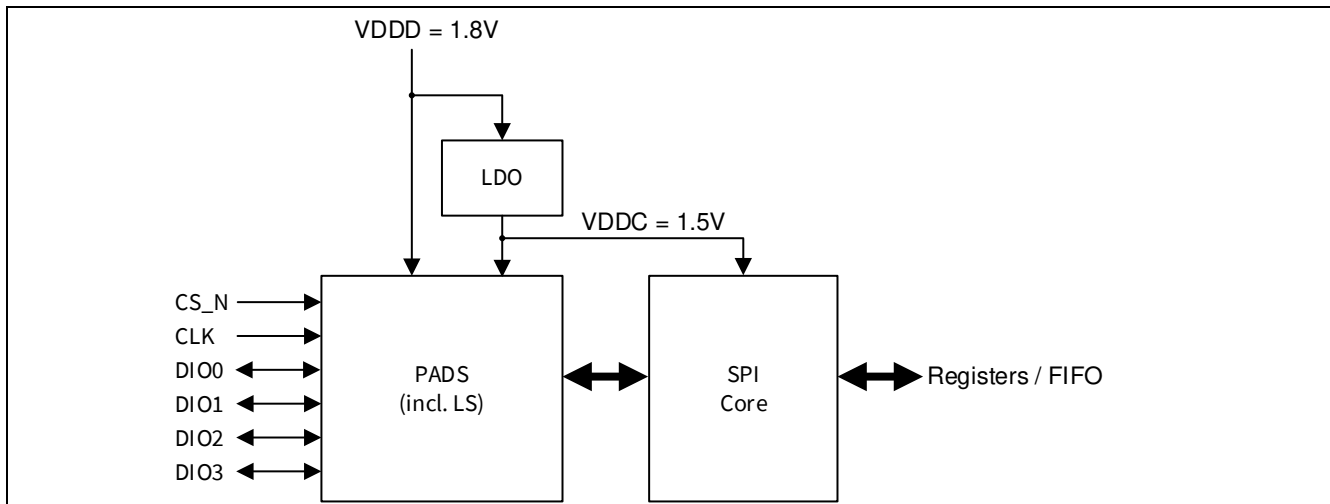
Figure 48 SPI module
