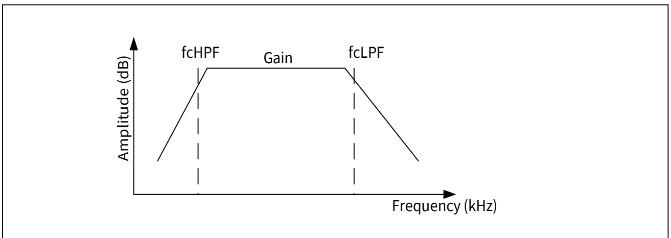
Figure 73 Baseband characteristic
