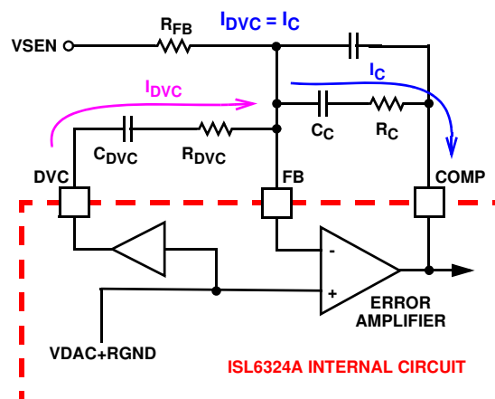
FIGURE 9. DYNAMIC VID COMPENSATION NETWORK
