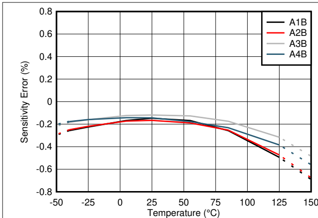
Figure 7-1. TMCS1101AxB Sensitivity Error vs Temperature
