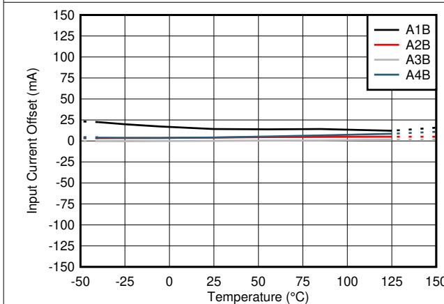
Figure 7-3. TMCS1101AxB Input Offset Current vs Temperature
