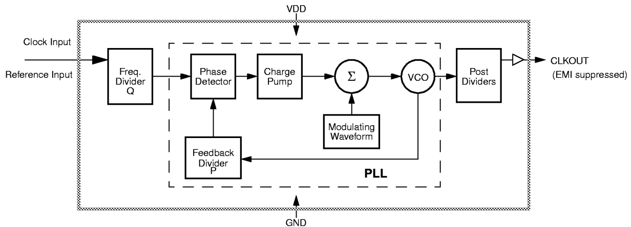
Figure 1. System Block Diagram (Concept, not actual implementation)
