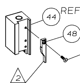
POST-FEED 1 1/8 STROKE
