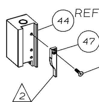
POST-FEED 1 5/8 STROKE
