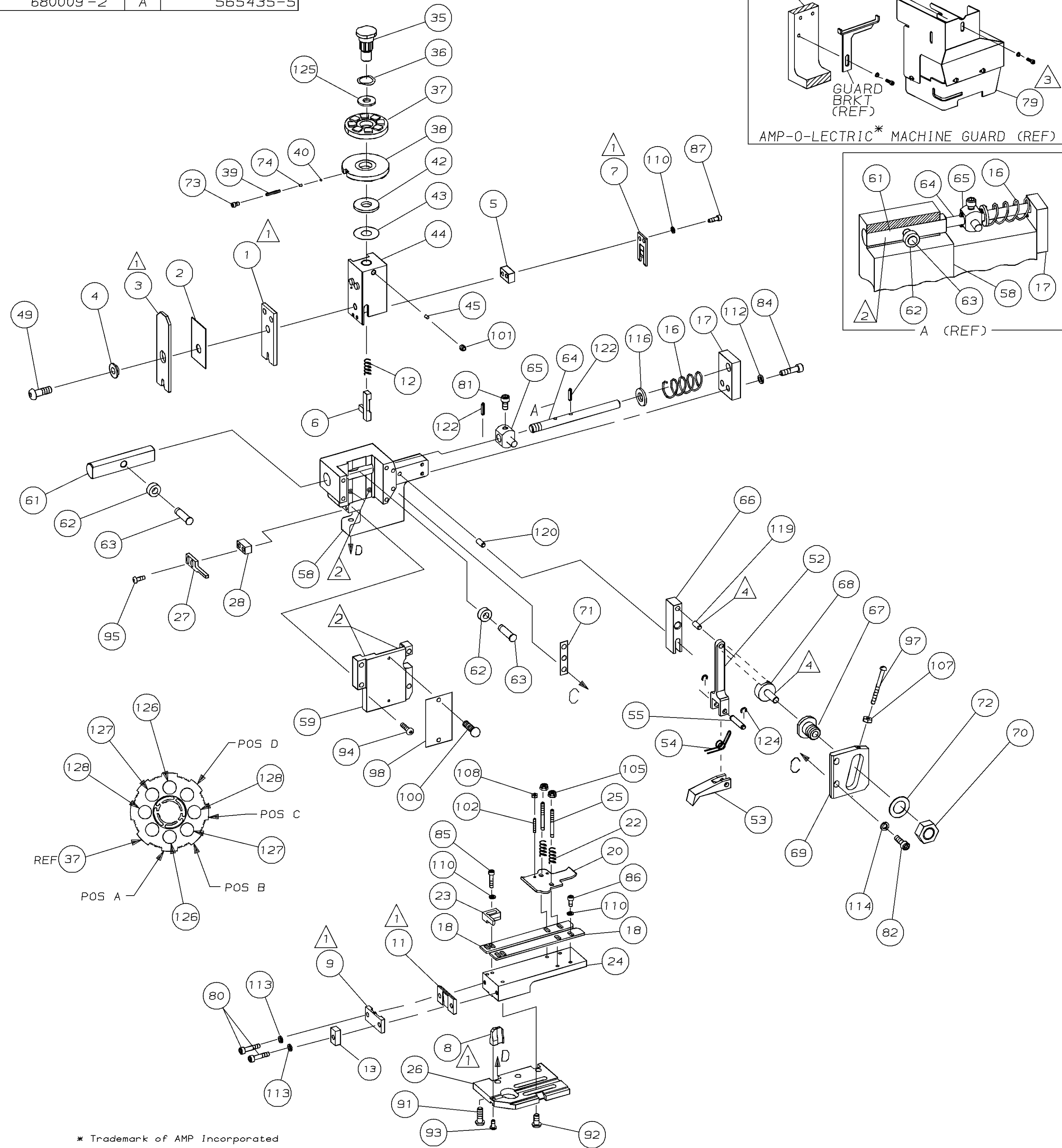
POST-FEED 1 5/8 STROKE
