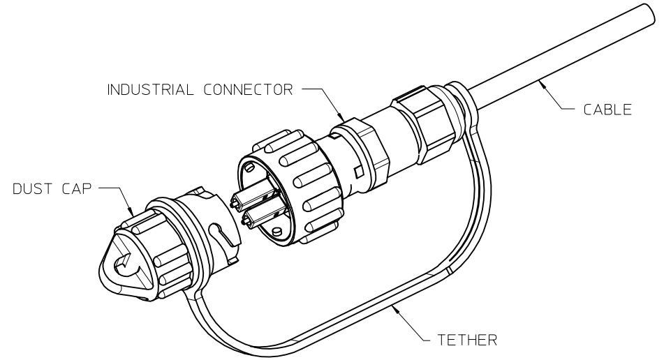
ISOMETRIC VIEW (LC INDUSTRIAL CONNECTOR SHOWN)
