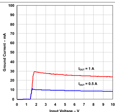
Figure 6. Ground Current vs Input Voltage T_J = 25\text{ °C} V_{EN} = V_{IN} V_{OUT} = 1.21\text{ V} TPS73801
