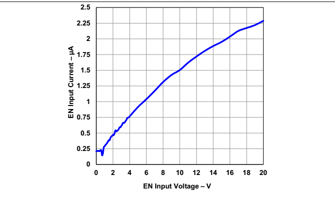
Figure 10. EN Input Current vs EN Input Voltage
