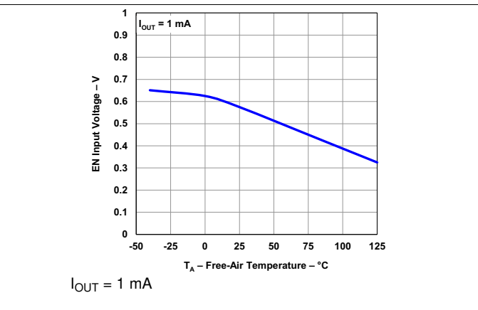
Figure 12. EN Threshold (On to Off) vs Temperature
