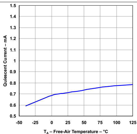
Figure 3. Quiescent Current vs Temperature V_{IN} = 6\text{ V} V_{EN} = V_{IN} I_{OUT} = 0\text{ A} TPS73801
