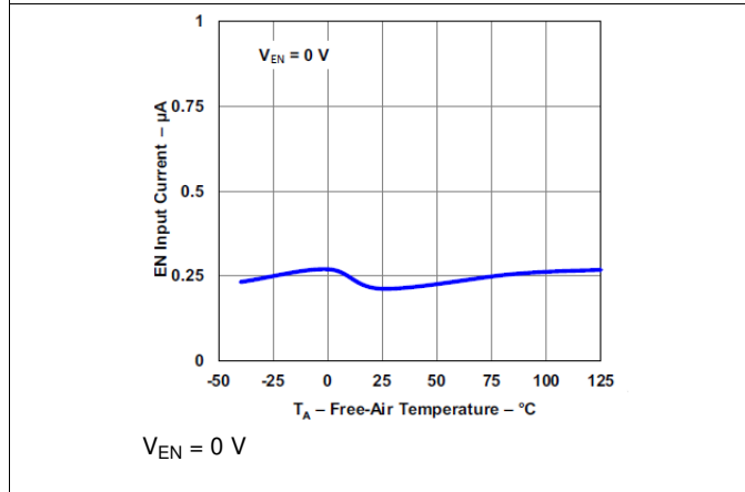
Figure 9. EN Input Current vs Temperature
