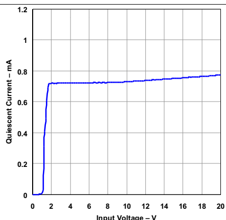
Figure 5. Quiescent Current vs Input Voltage T_J = 25\text{ °C} V_{EN} = V_{IN} R_{OUT} = 4.3\text{ k}\Omega TPS73801
