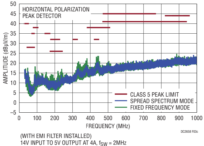
Figure 3. LT8643S Demo Circuit DC2658A EMI Performance (14V Input from V IN_EMI , with EMI Filter, I OUT = 4A)
