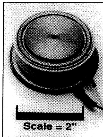
T9G0 1000A Phase Control SCR 1000 Amperes Average, 2400 Volts
