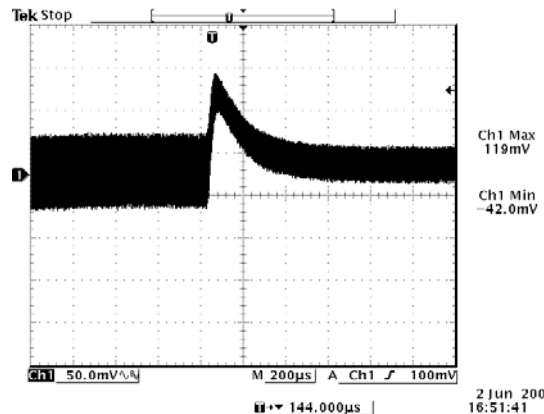
100% to 50% load transient at V_{in}=3.3 V, V_o=15 V
