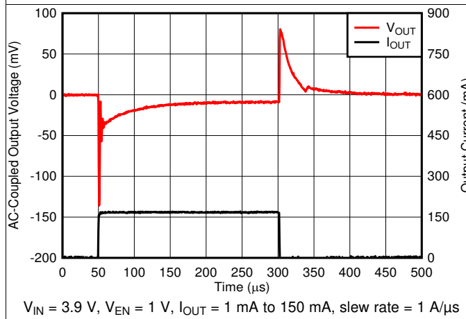
Figure 21. Load Transient
