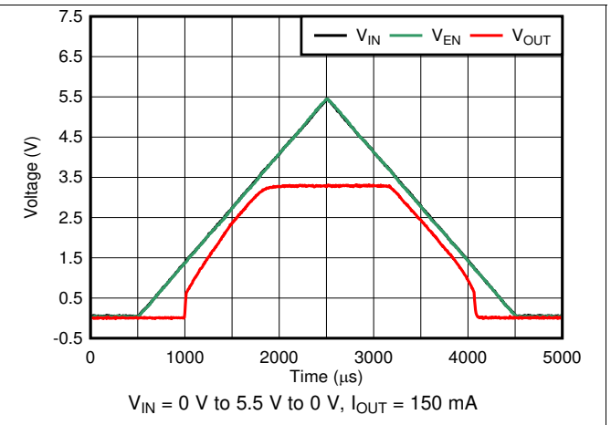
Figure 26. Start-Up and Shutdown
