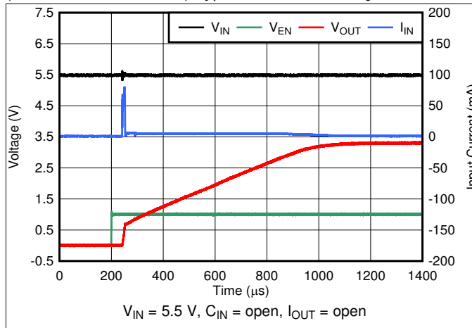
Figure 25. Start-Up With EN, Inrush Current
