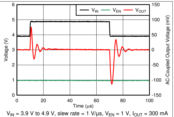
Figure 20. Line Transient
