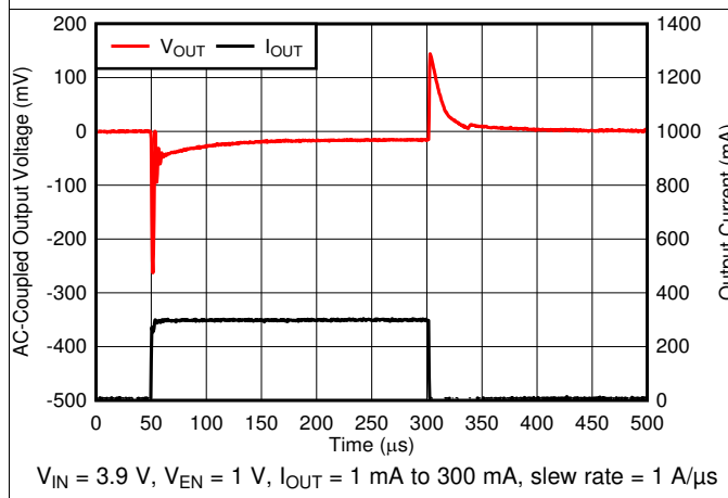
Figure 23. Load Transient
