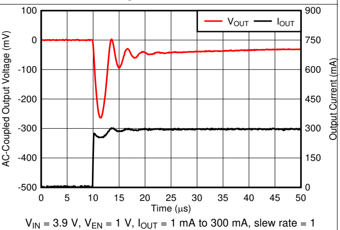
Figure 22. Load Transient
