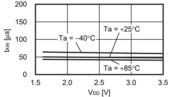
2.6 Awake mode time ( t_{AW} ) vs. Power supply voltage ( V_{DD} )
