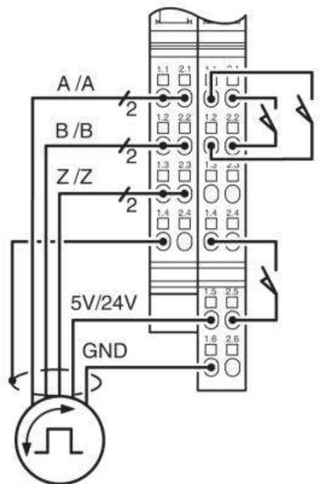
Connection diagram
