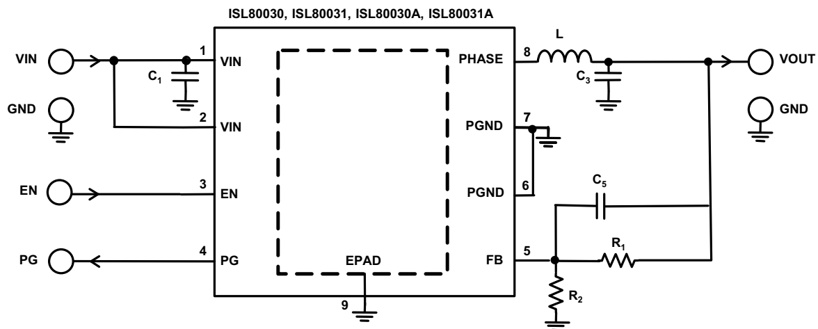
FIGURE 1. BLOCK DIAGRAM
