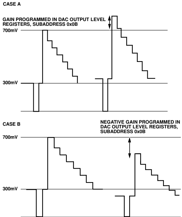
Figure 70. Programmable DAC Gain—Positive and Negative Gain
