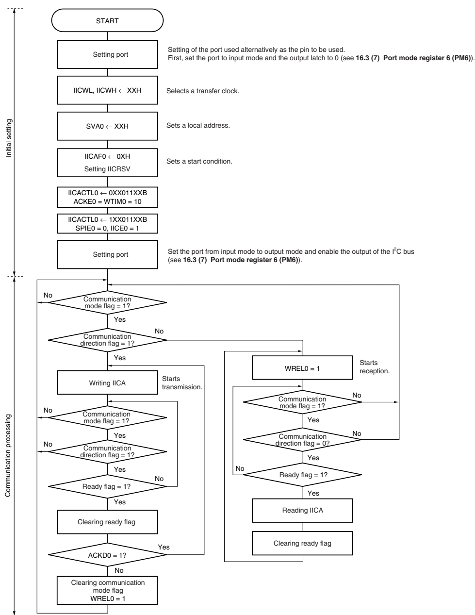
Figure 16-30. Slave Operation Flowchart (1)
