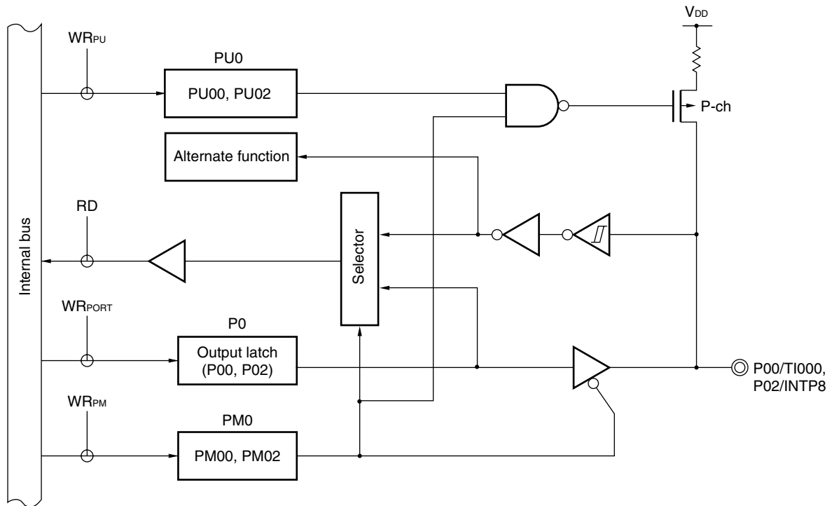
Figure 4-1. Block Diagram of P00, P02
