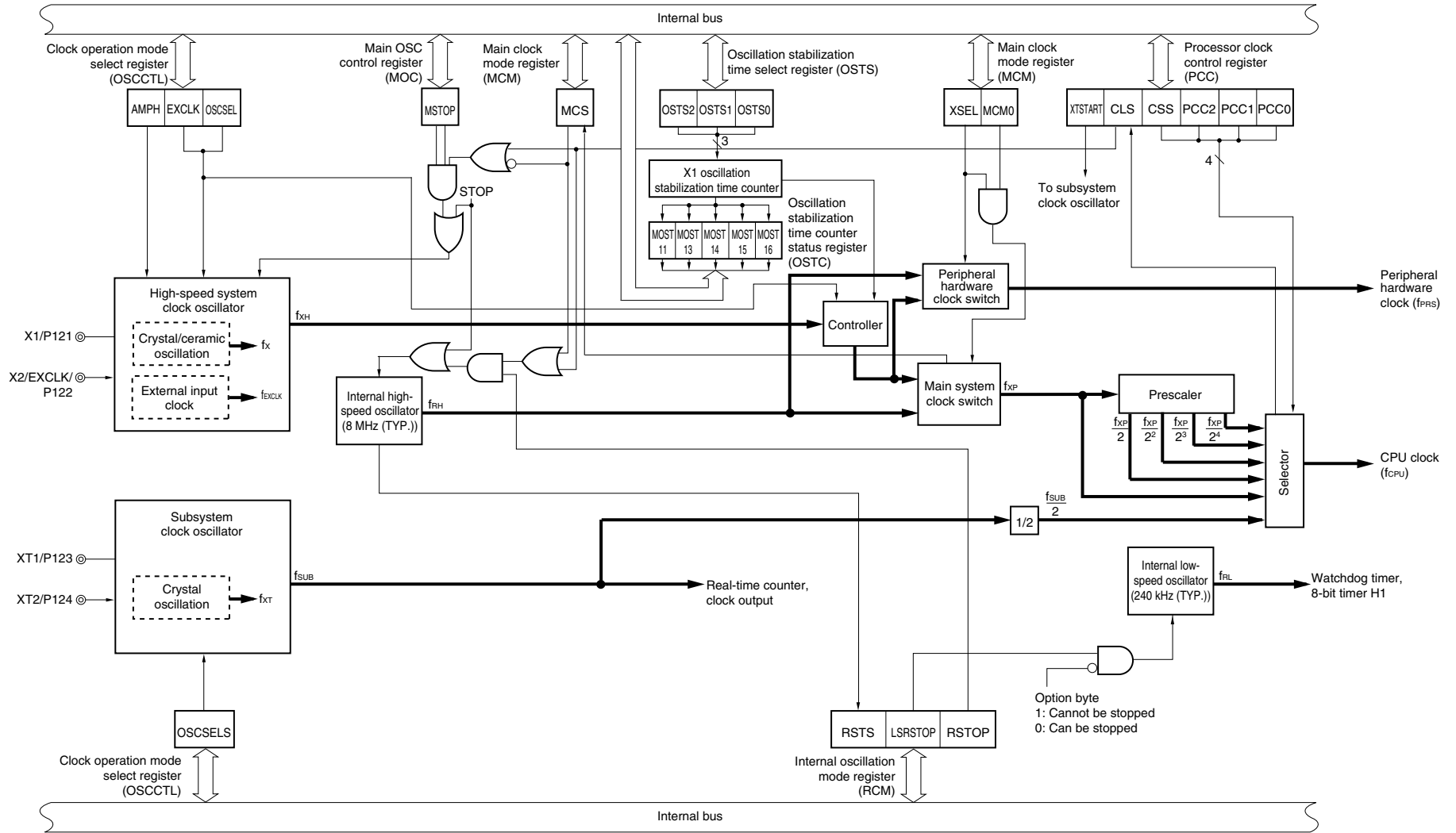
Figure 5-2. Block Diagram of Clock Generator (78K0/KC2-A (48 pins))
