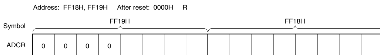
Figure 12-8. Format of 12-Bit A/D Conversion Result Register (ADCR)
