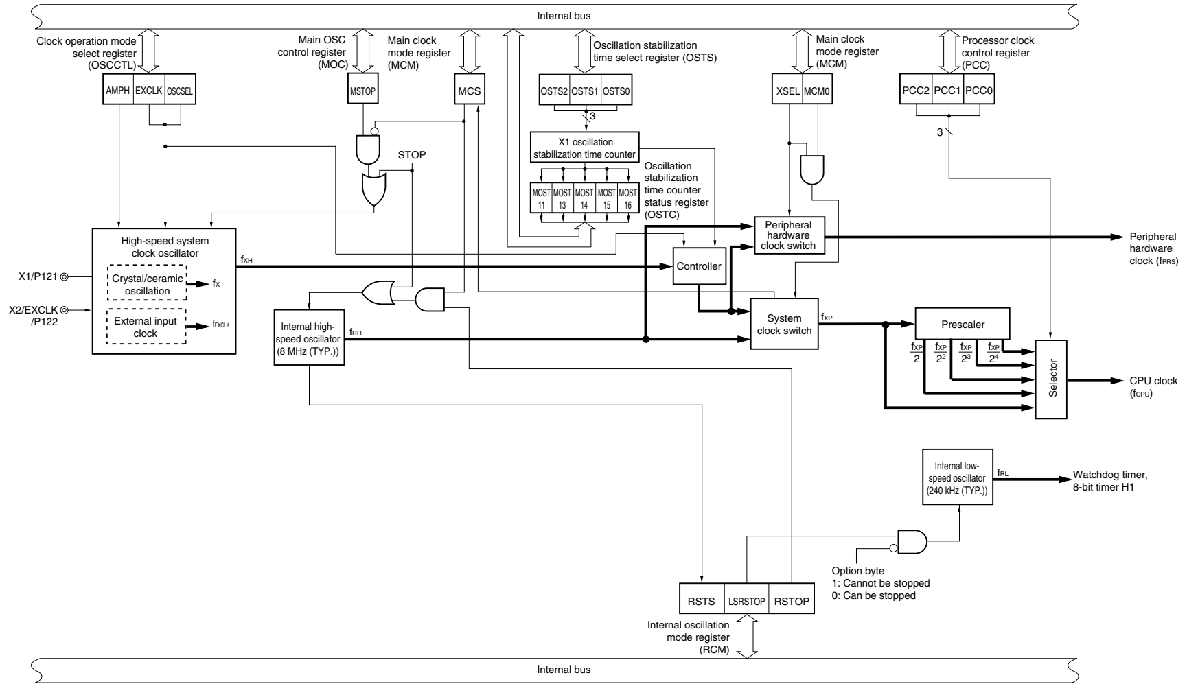
<R> Figure 5-1. Block Diagram of Clock Generator (78K0/KB2-A, 78K0/KC2-A (36 pins))
