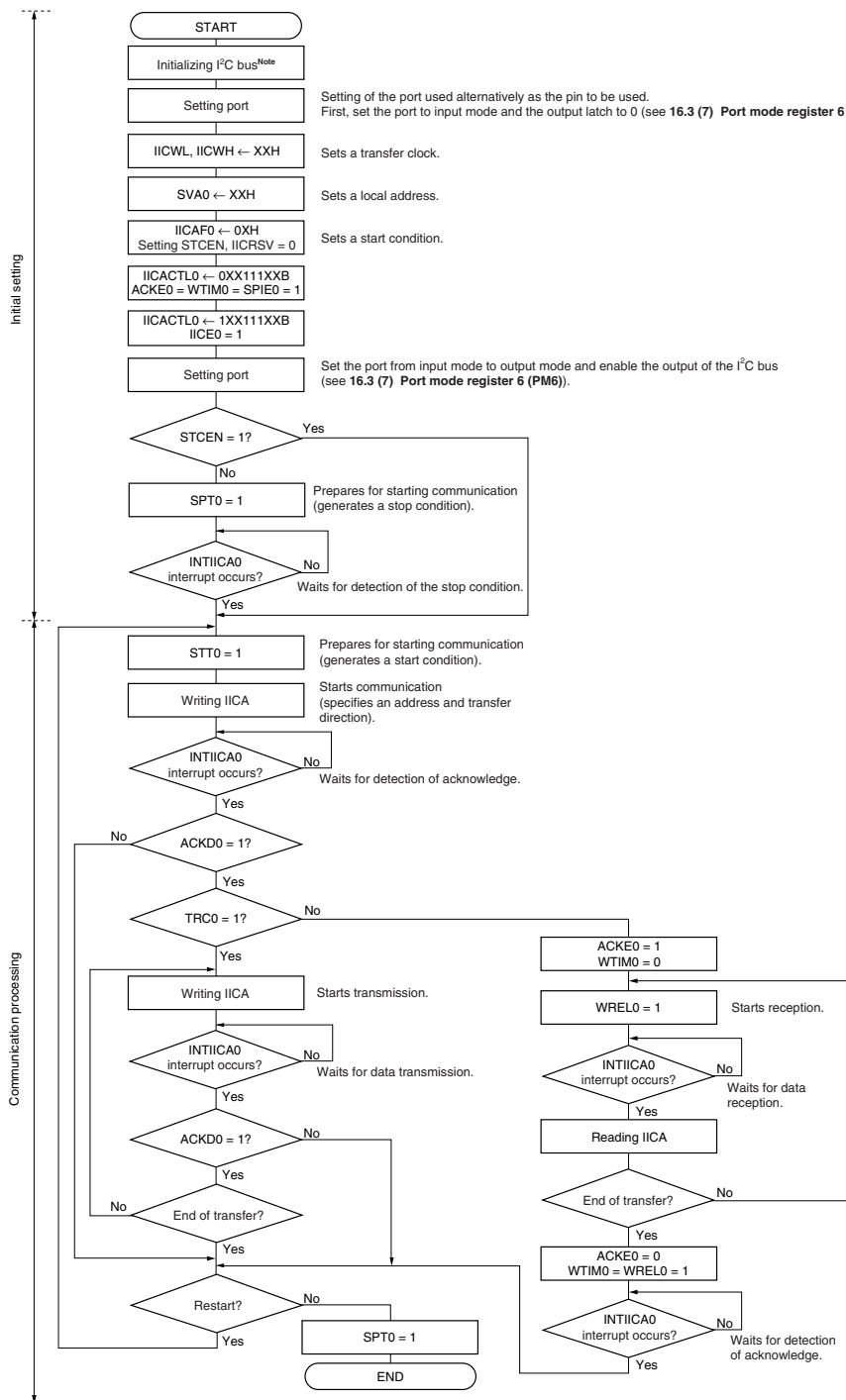
Figure 16-28. Master Operation in Single-Master System
