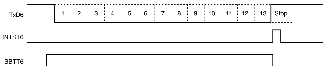
Figure 14-22. SBF Transmission
