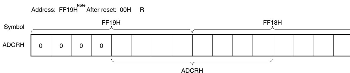
Figure 12-9. Format of 8-Bit A/D Conversion Result Register (ADCRH)
