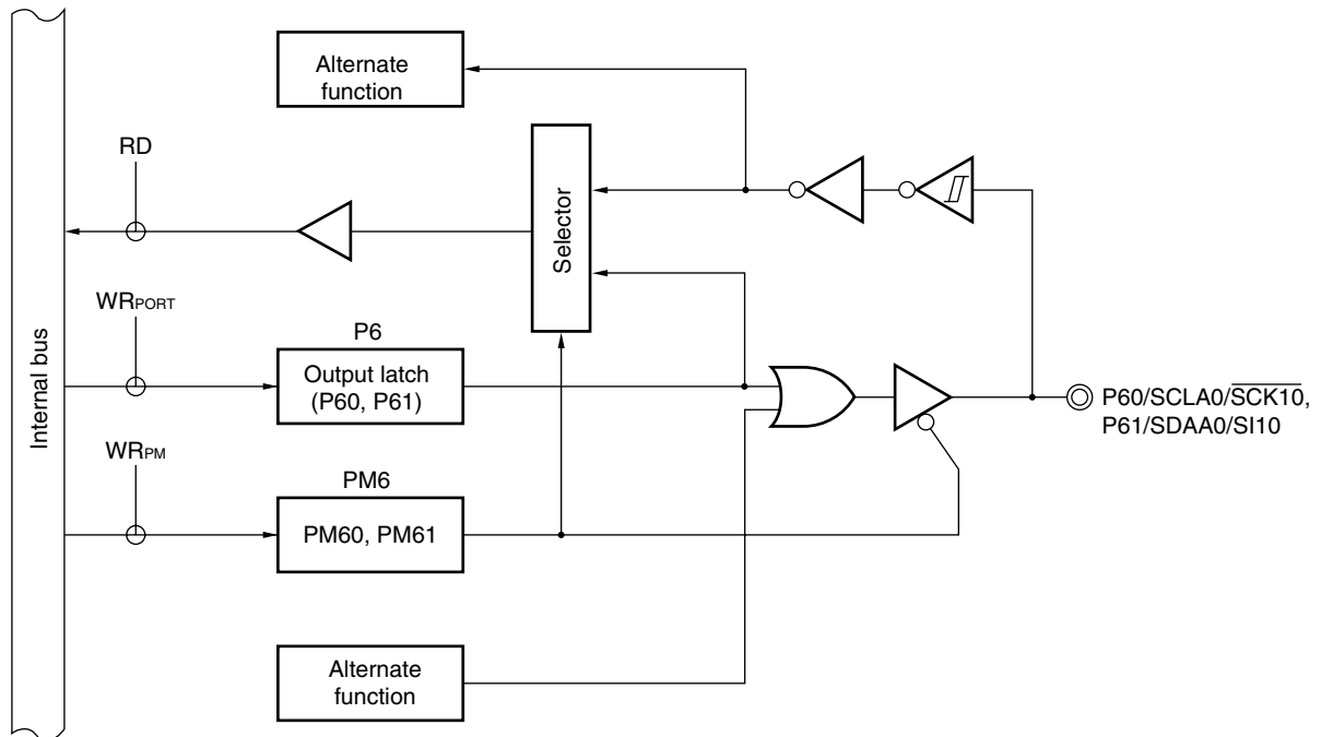
Figure 4-16. Block Diagram of P60 and P61
