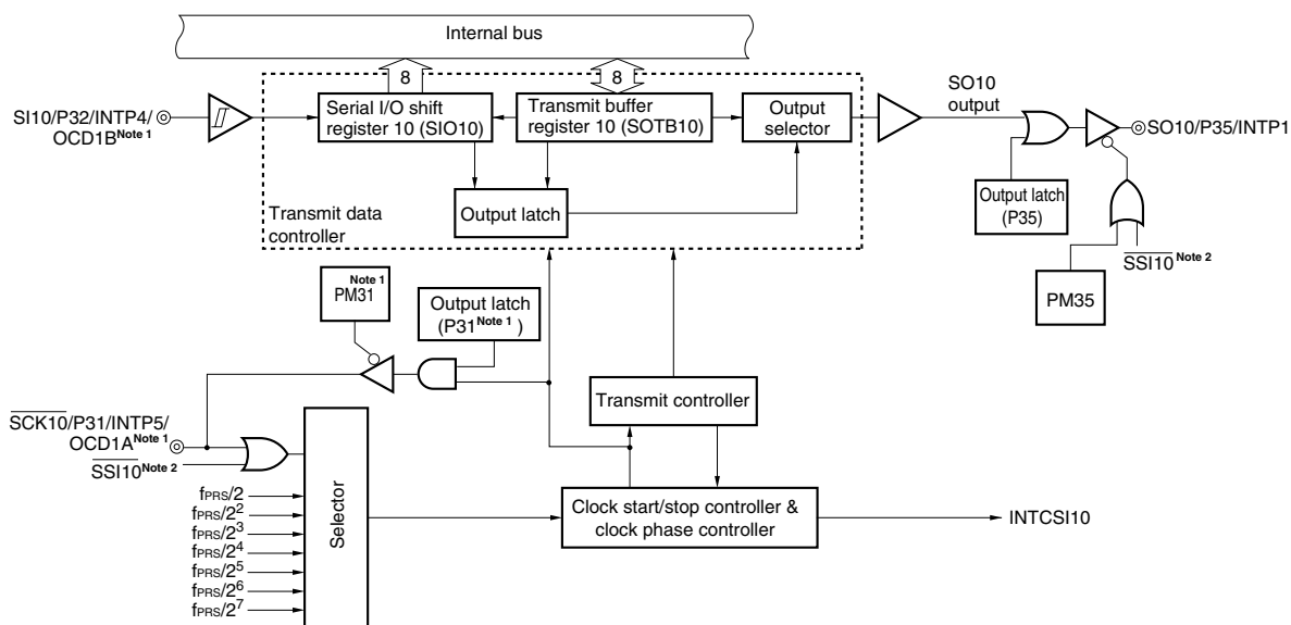
Figure 15-1. Block Diagram of Serial Interface CSI10
