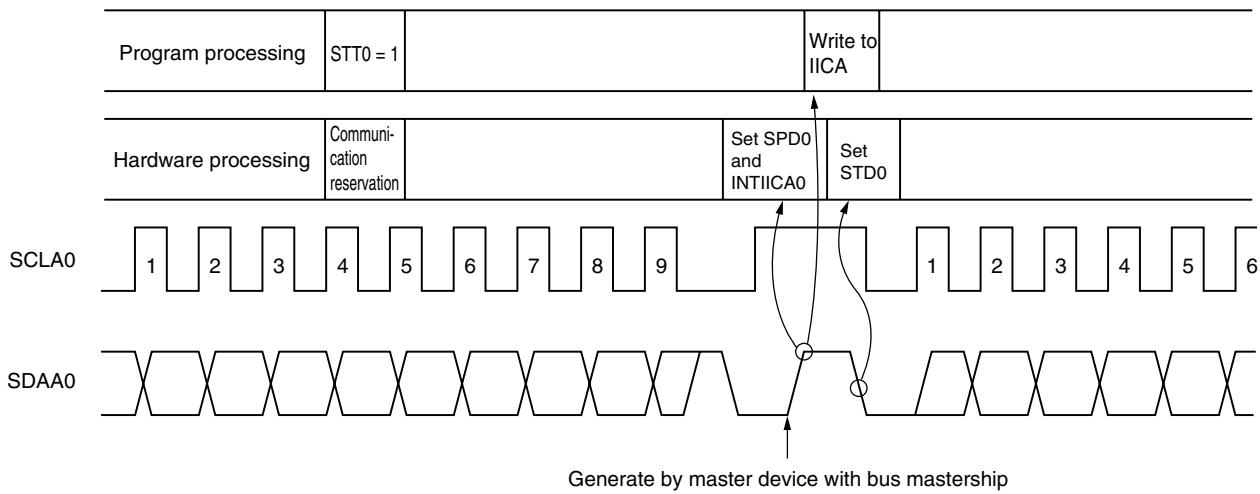
Figure 16-25. Communication Reservation Timing
