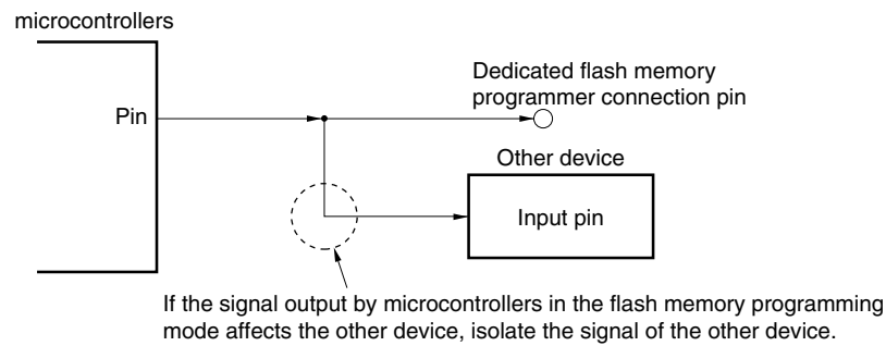
Figure 25-7. Malfunction of Other Device
