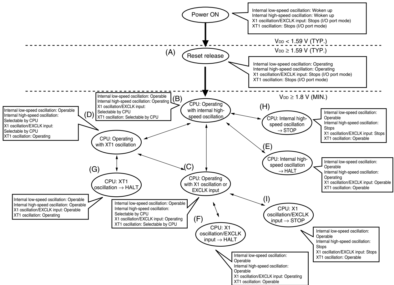
Figure 5-16. CPU Clock Status Transition Diagram (When 1.59 V POC Mode Is Set (Option Byte: POCMODE = 0)) (78K0/KC2-A (48 pins))
