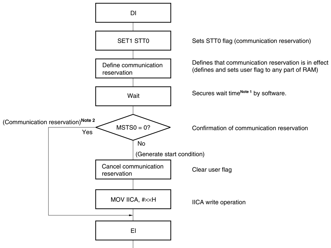
Figure 16-27. Communication Reservation Protocol
