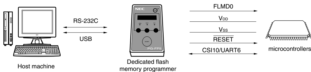
Figure 25-2. Environment for Writing Program to Flash Memory
