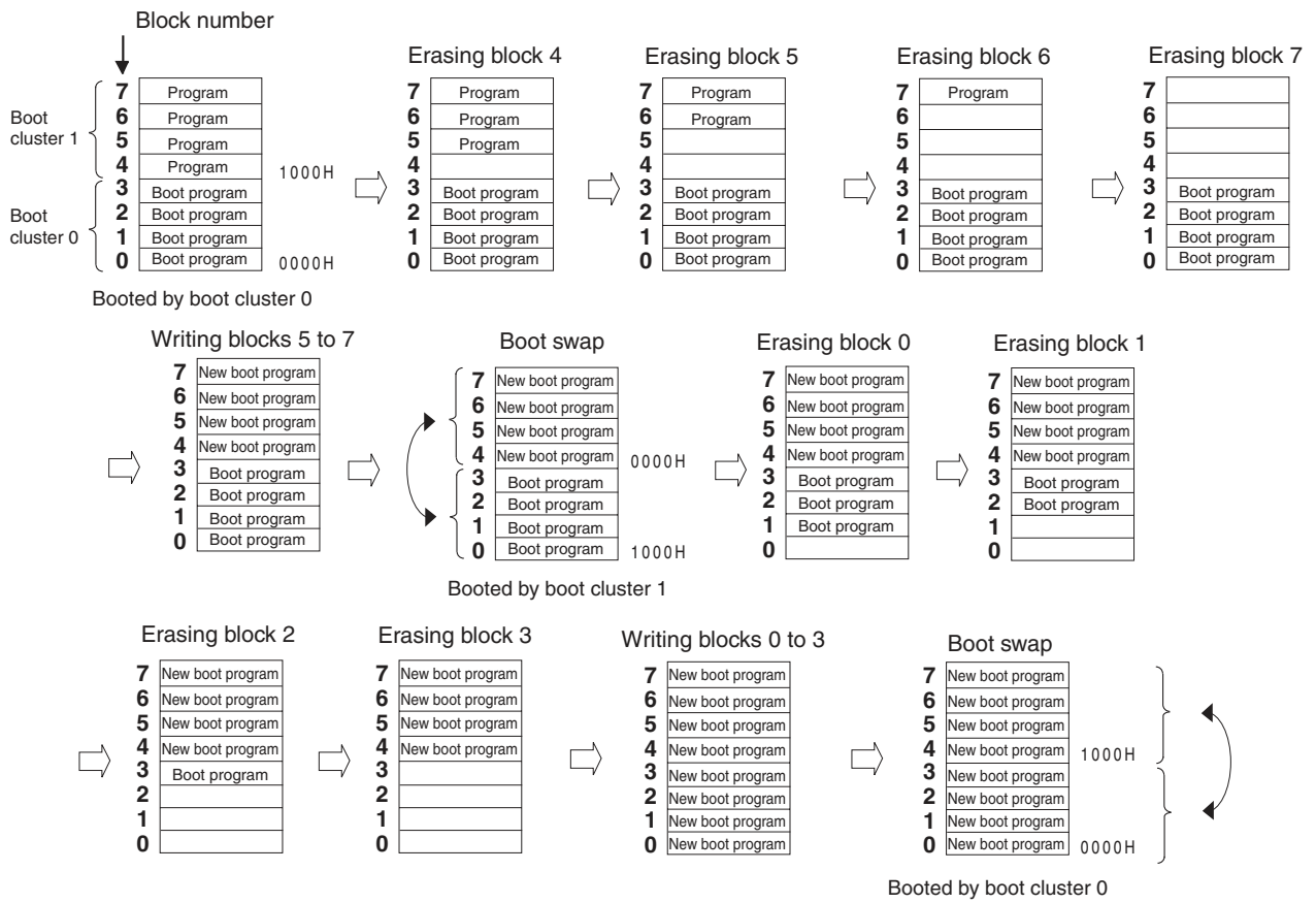
Figure 25-15. Example of Executing Boot Swapping
