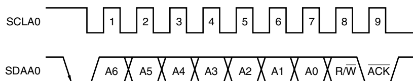
Figure 16-17. \overline{\text{ACK}}
