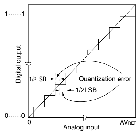
Figure 12-20. Quantization Error
