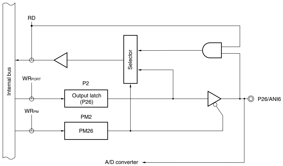
Figure 4-9. Block Diagram of P26
