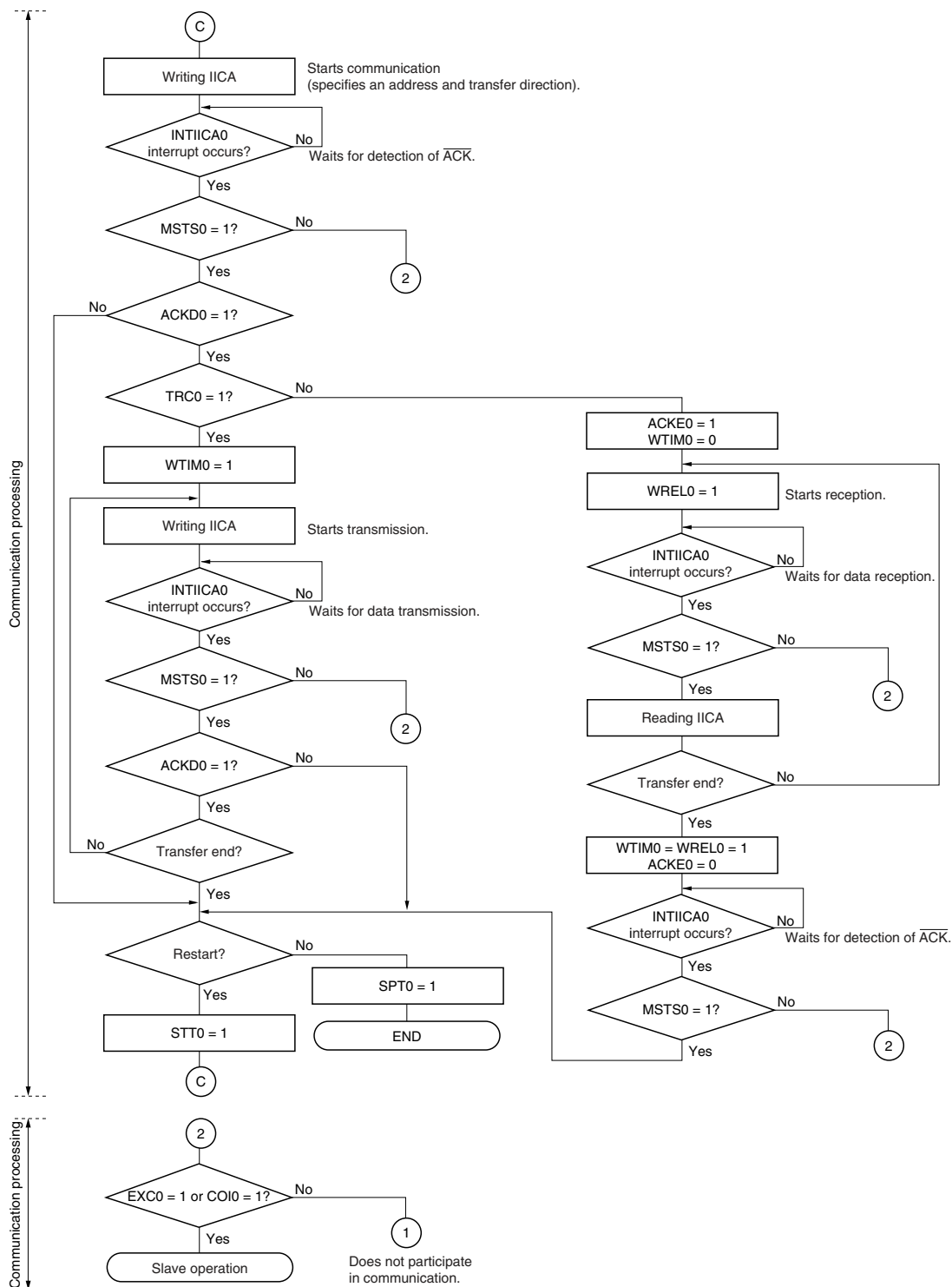
Figure 16-29. Master Operation in Multi-Master System (3/3)
