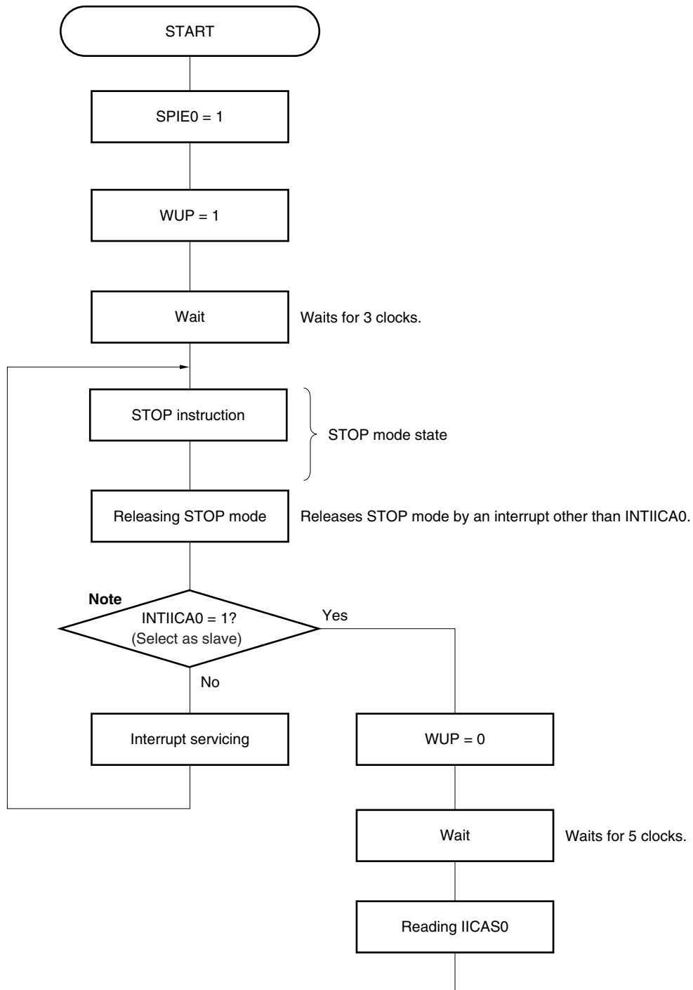
Figure 16-24. To Specify IICA as Master After STOP Mode Is Released by Other Than INTIICA (If IICA Does Not Have to Operate as Master)
