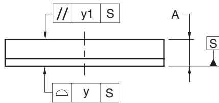
DETAIL (C)
