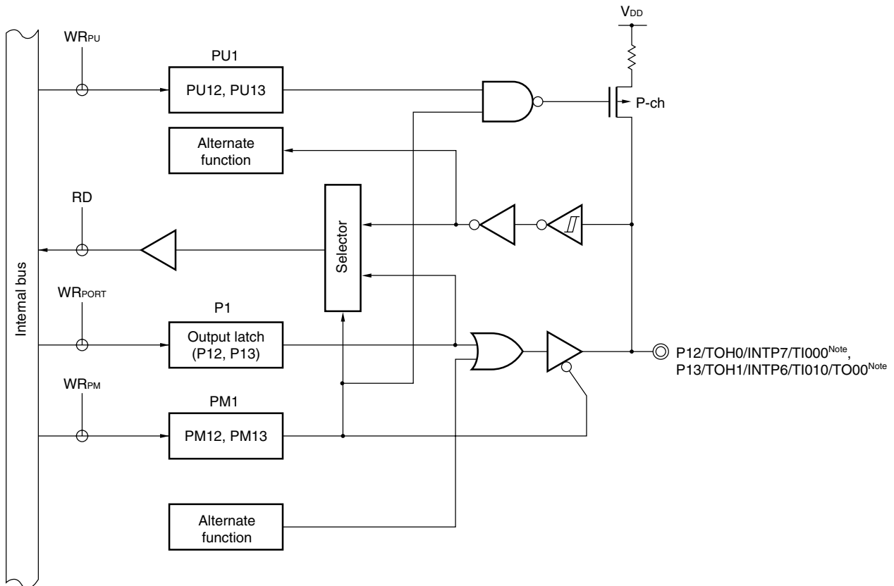
Figure 4-5. Block Diagram of P12 and P13
