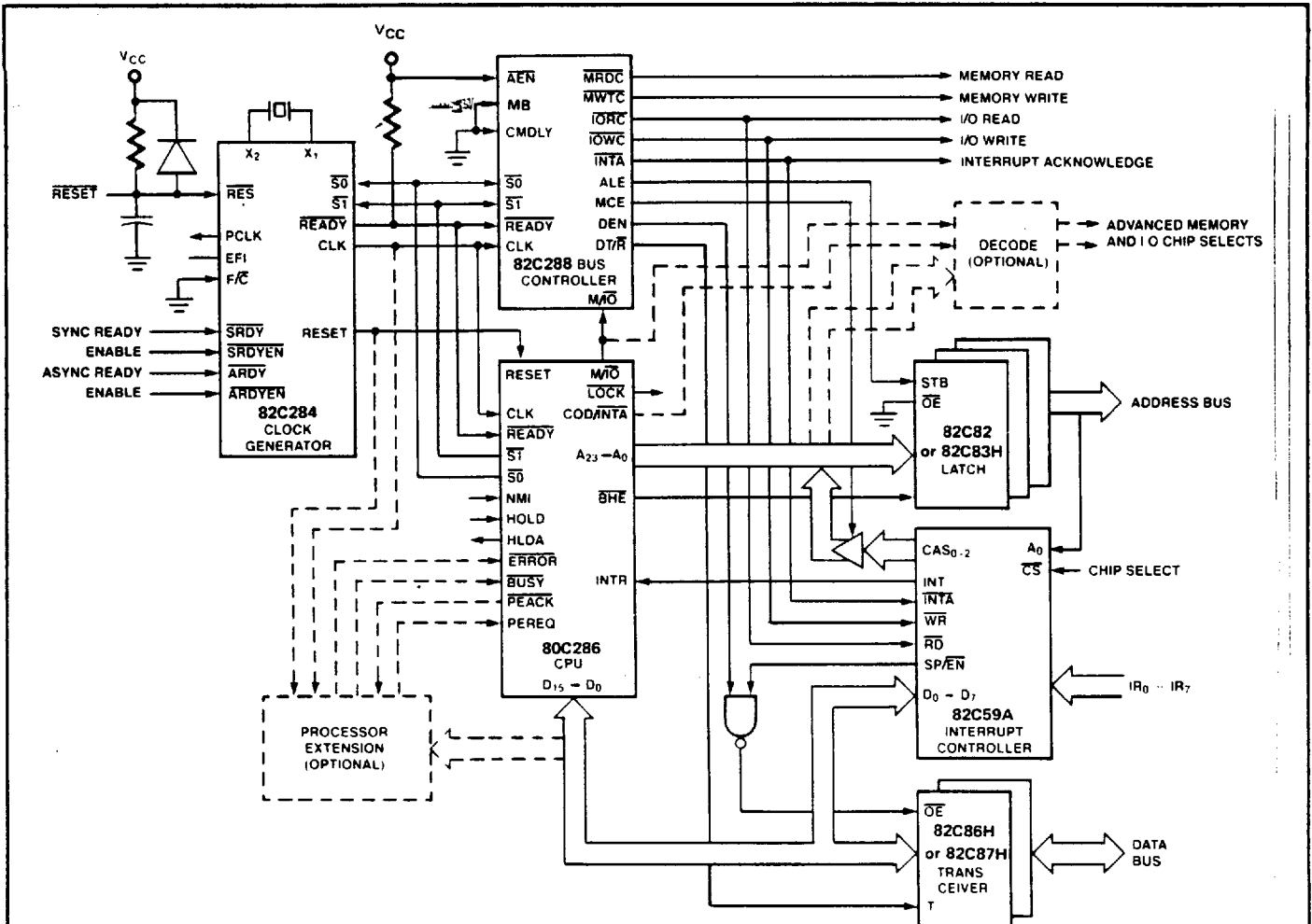
FIGURE 31. BASIC 80C286 SYSTEM CONFIGURATION
