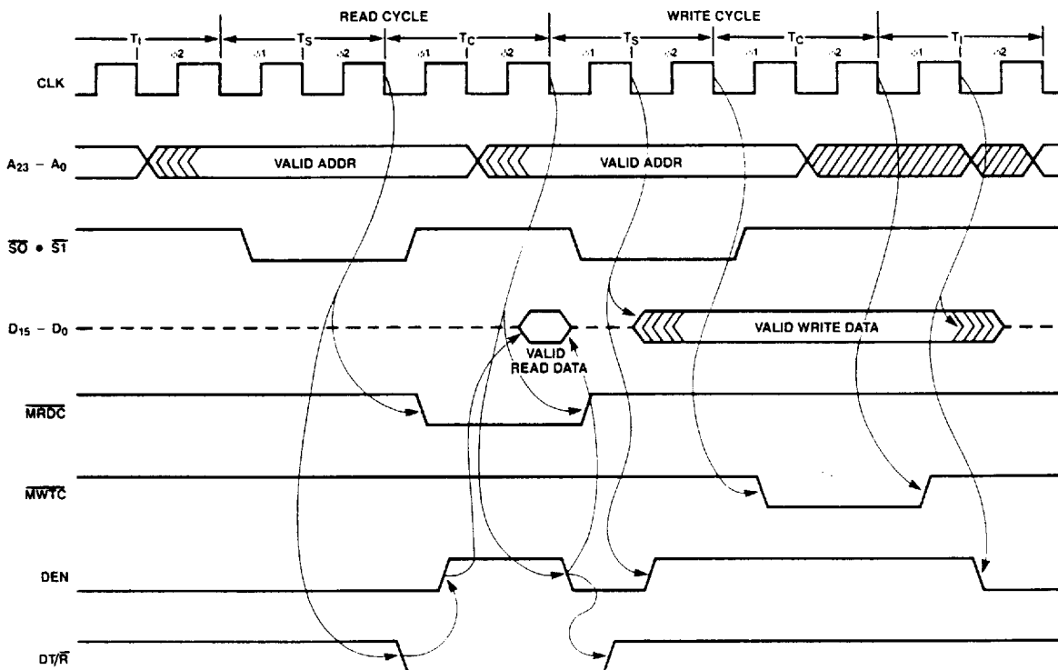
FIGURE 26. BACK TO BACK READ-WRITE CYCLE
