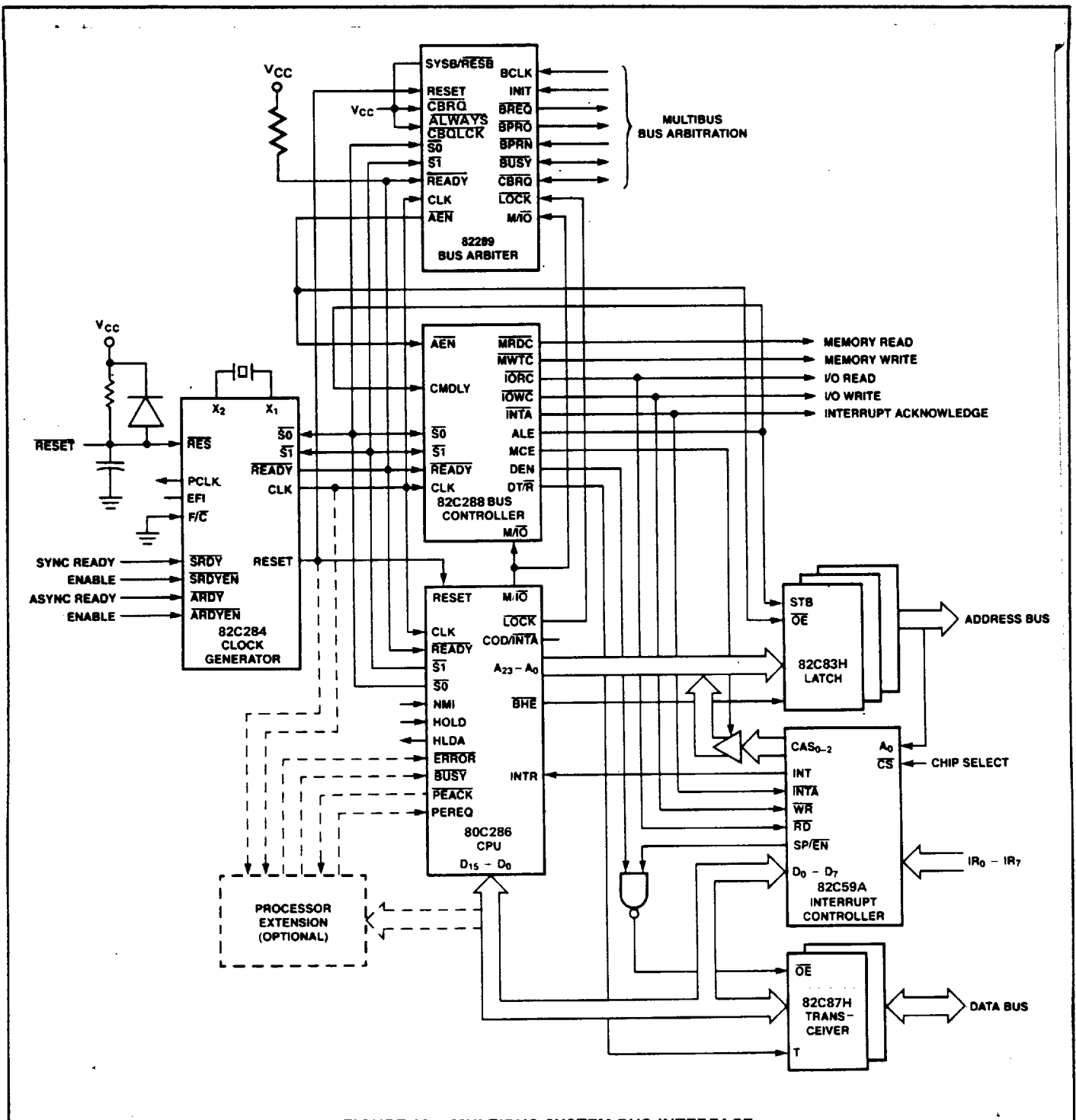
FIGURE 32. MULTIBUS SYSTEM BUS INTERFACE
