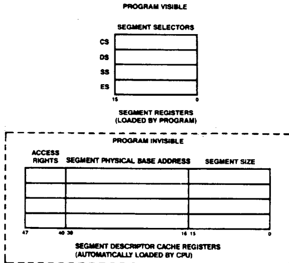
FIGURE 13. DESCRIPTOR CACHE REGISTERS
