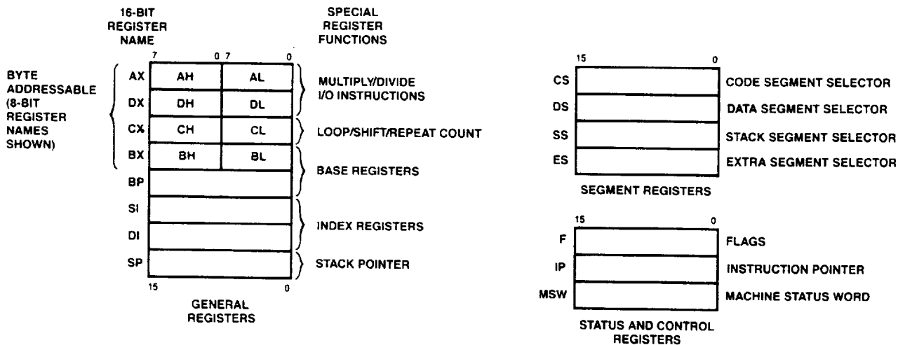
FIGURE 1. REGISTER SET
