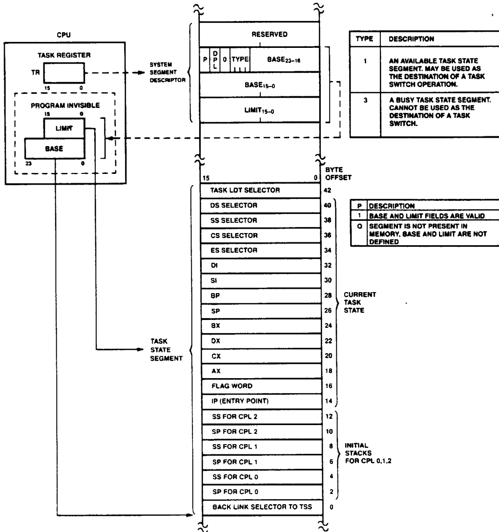
FIGURE 19. TASK STATE SEGMENT AND TSS REGISTERS
