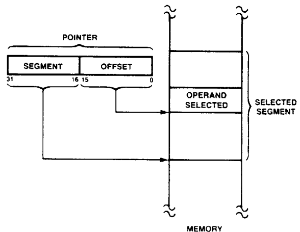
FIGURE 4. TWO COMPONENT ADDRESS
