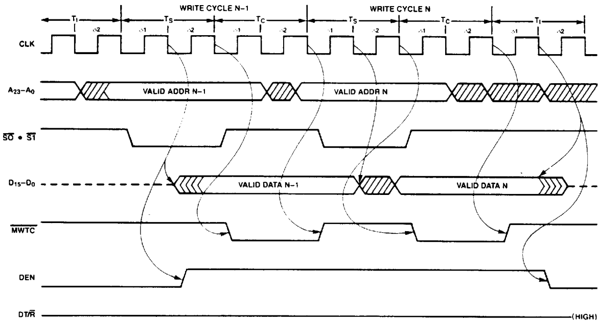
FIGURE 28. BACK TO BACK WRITE-WRITE CYCLE
