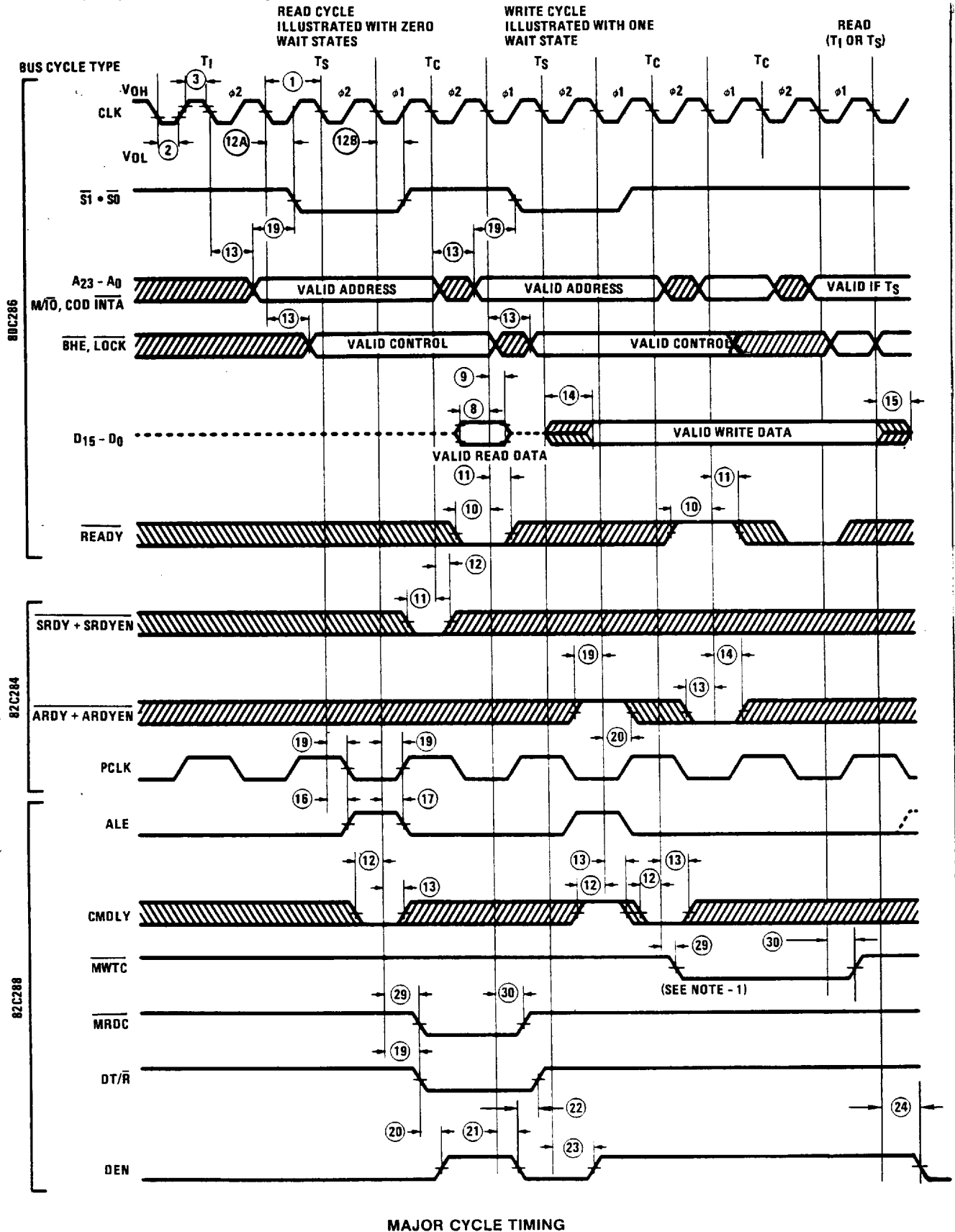
MAJOR CYCLE TIMING
