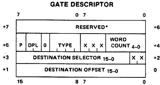
GATE DESCRIPTOR FIELDS
