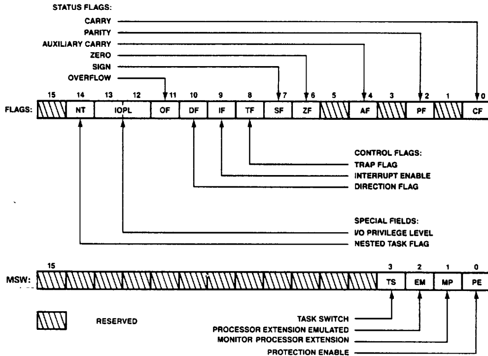
FIGURE 2. STATUS AND CONTROL REGISTER BIT FUNCTIONS
