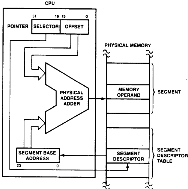
FIGURE 9. PROTECTED MODE MEMORY ADDRESSING
