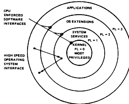
FIGURE 18. HIERARCHICAL PRIVILEGE LEVELS
