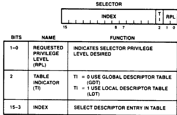
FIGURE 14. SELECTOR FIELDS
