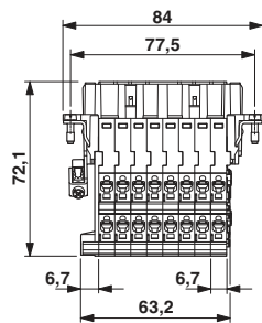
Dimensional drawing
