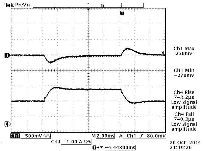
Figure 10. Vout = 54 V, 75%-50% Load Transients at Vin = 72 V, Ta=25°C
