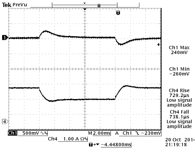
Figure 9. Vout = 54 V, 50%-75% Load Transients at Vin = 72 V, Ta=25°C
