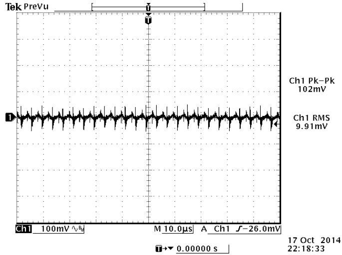
Figure 8. Ripple and noise 72 Vdc input, 54 Vdc/3 A output Ta=25°C, and with a 0.1 uF ceramic cap and 220 uF electrolytic cap at output
