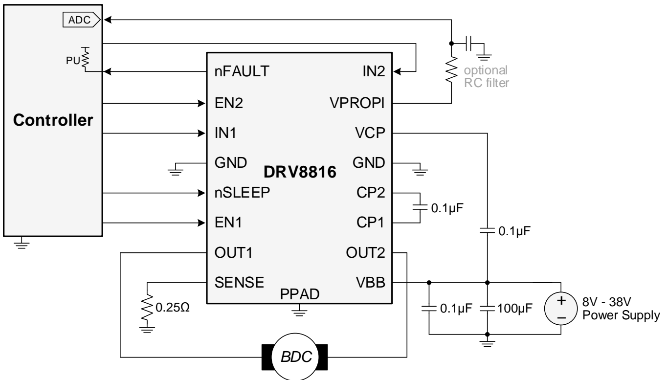
Figure 7. Typical Application
