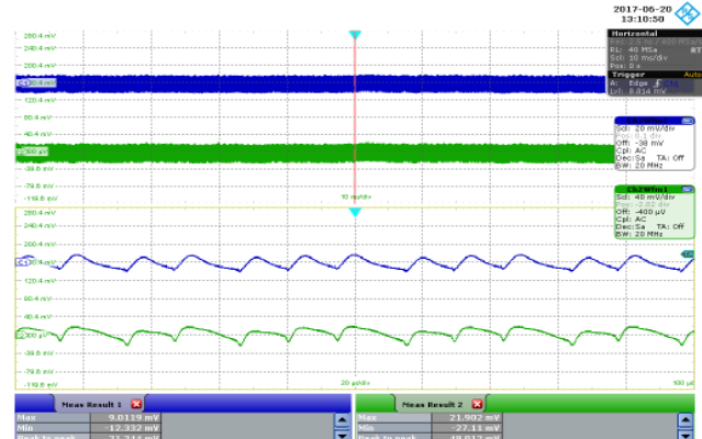
Figure 53 – Output Ripple Voltage Waveforms. 265 VAC Input. 5 V PK : 22 mV, 12 V PK : 50 mV. Upper: 5 V, 20 mV / div. Lower: 12 V, 40 mV /, 10 ms, 20 μs / div.
