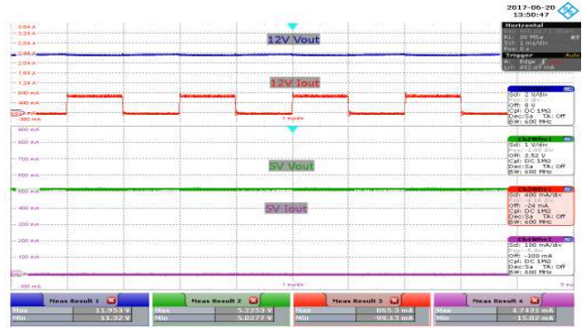
Figure 25 – 0 A – 0.7 A, 12 V Load Step Transient Response. 265 VAC. 5 V MIN : 5.02 V.; 5 V MAX : 5.22 V. 12 V MIN : 11.32 V.; 12 V MAX : 11.95 V. Upper: 12 V OUT , 2 V / div. Upper Middle: 12 V I OUT . 400 mA / div. Upper Middle: 5 V OUT , 1 V / div. Lower: 5 V I OUT , 100 mA / div., 1 ms / div.
